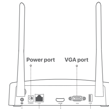
Grounding terminal 10/100 Mbps auto-negotiation Ethernet port HDMI port VGA port USB2.0 port
